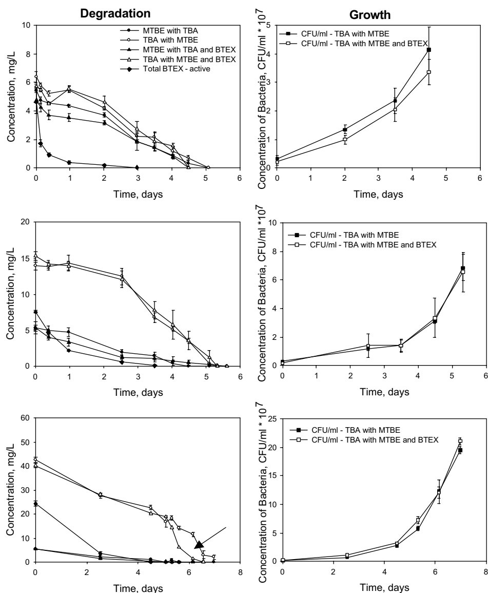
Figure 3. Plots of TBA degradation and growth (with MTBE initially present at 5 mg/l in all studies) at three initial concentration levels: 6, 15, and 40–42 mg/l, with and without BTEX provided at half the molar concentration. For brevity, controls not plotted. Arrow indicates evidence of faster ultimate TBA degradation rate when BTEX present initially.
