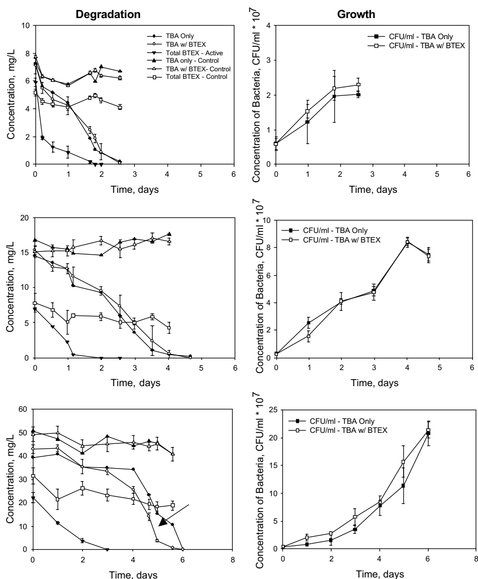
Figure 2. Plots of TBA degradation and growth at three initial concentration levels: 7, 15, and 40–42 mg/l, with and without BTEX. Arrow indicates evidence of faster ultimate TBA degradation rate when BTEX present initially.
