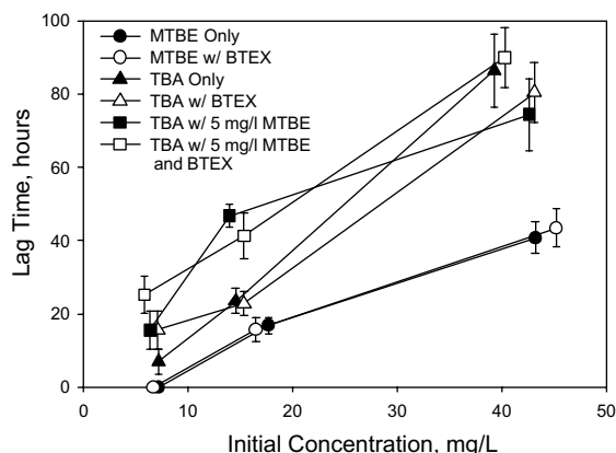
Figure 5. Plots of degradation lag observed versus Initial concentration (MTBE or TBA). Error bars indicate standard deviation of triplicate samples.
