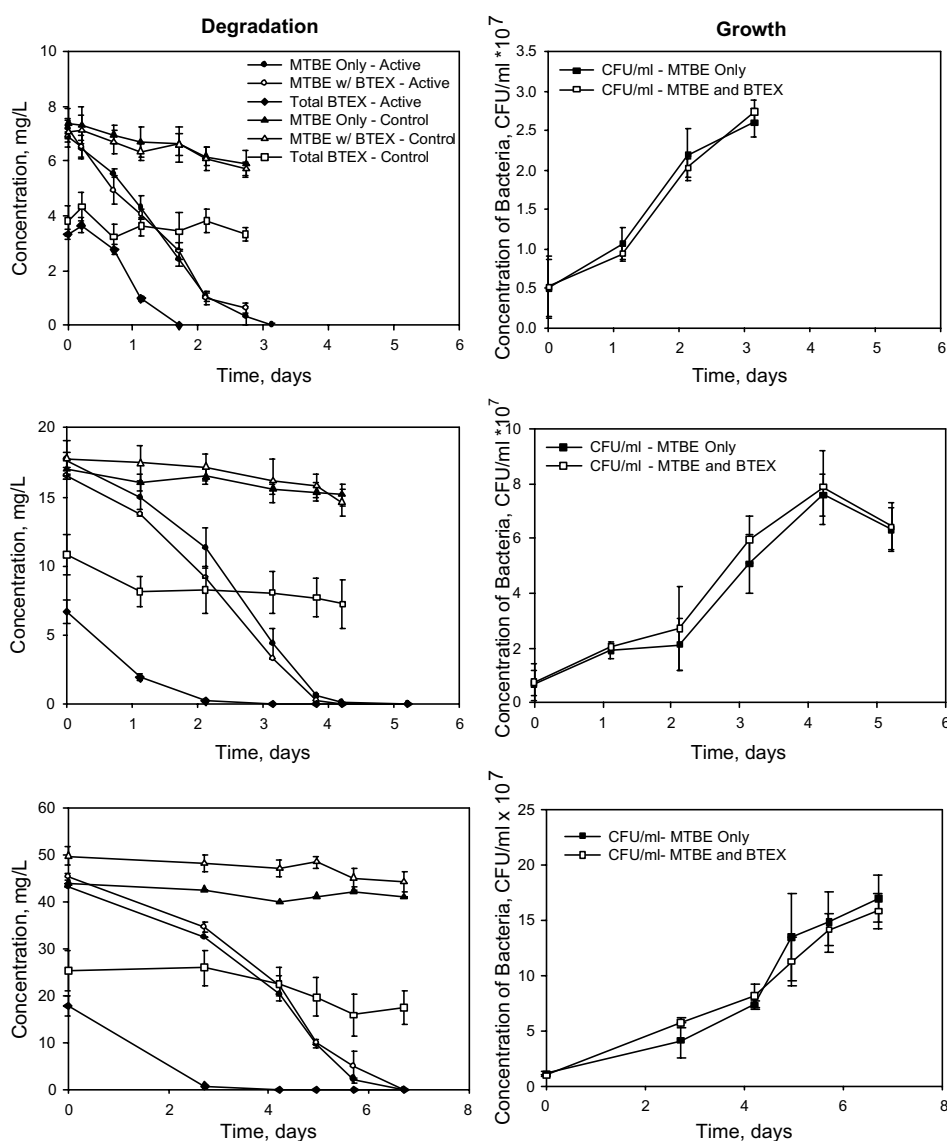
Figure 1. Plots of MTBE degradation and growth at three initial concentration levels: 7, 17 mg/l, and 44–45 mg/l, with and without BTEX present. TBA was not observed to be present as an intermediate.
