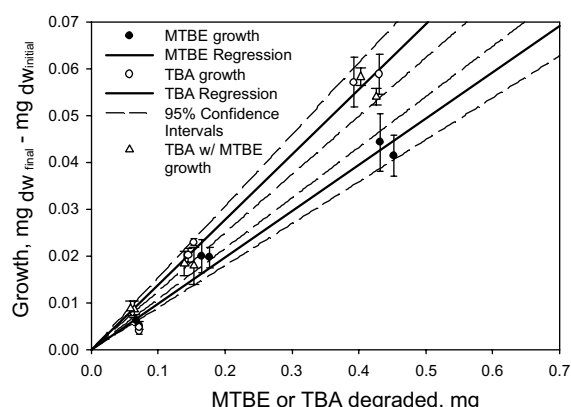
Figure 6. Linear regression of growth (mg dry weight) versus mass (mg) of MTBE or TBA utilized. Dashed lines indicate 95% confidence intervals on the regression line estimates. TBA growth with 5 mg/l MTBE present (triangles) is also plotted, but not included in the regression analysis.
