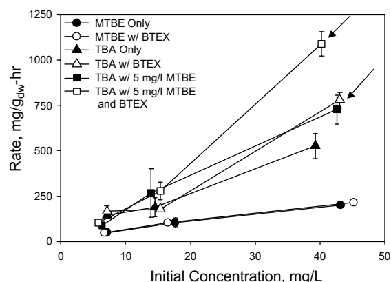
Figure 4. Plots of rate versus Initial concentration for MTBE and TBA. Error bars indicate standard deviation of triplicate samples. Arrows indicate evidence of faster TBA degradation rate when BTEX present initially at the highest concentration.
